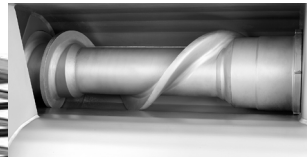
Worm/auger shown mounted in the SuperGrind 400/260 cabinet, top view.
