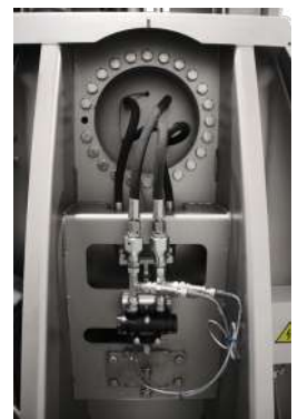
Pallet inverter seen from behind without cover, view of hydraulic unit and turning device.
